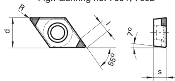
Fig.: Guhring no. 7691, 7692
