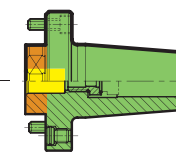
Shrink fit chucks Guhring no. 4760
