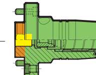
Hydraulic chucks Guhring no. 4360
