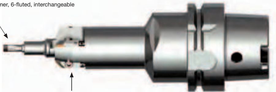
System GP 100 for machining valve seats, adjustable
