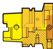
Alignment adaptor Guhring no. 4723
