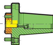
Shrink fit chucks Guhring no. 4717
