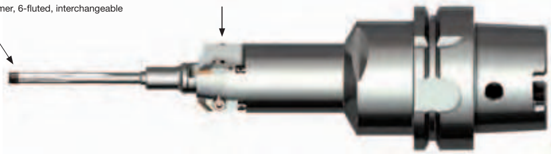
System GP 100 for machining valve seats, adjustable
