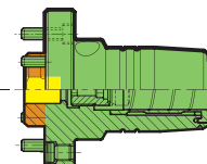
Hydraulic chucks Guhring no. 4722
