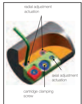
Fig. 8: OPERATION
