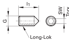
Fig.: Guhring no. 1689
